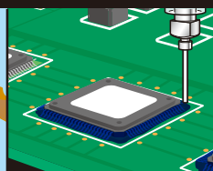
QFPへの防湿剤塗布 Seal coating for QFP package
